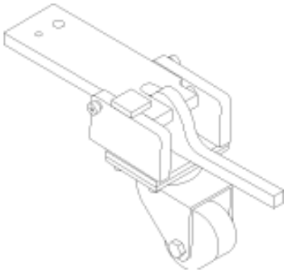
Wheel Assembly
